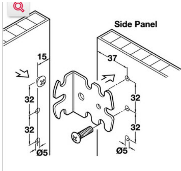
Satin chrome universal mounting bracket
